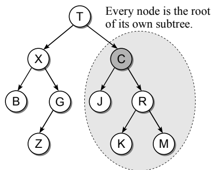
Figure 13.4: A subtree with root node C.
