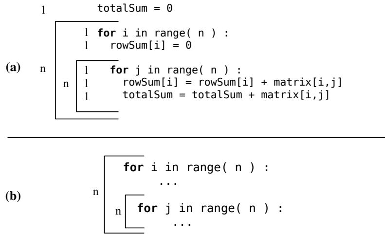
Figure 4.3: Markup for version one of the matrix summing algorithm: (a) shows all operations marked with the appropriate time and (b) shows only the non-constant time steps.
