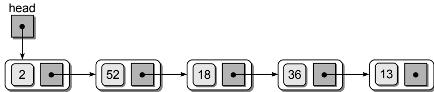
Figure 10.7: A sample singly linked list.
