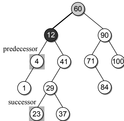
Figure 14.12: The logical successor and predecessor of node 12.
