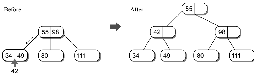
Figure 14.32: Splitting the root node is a special case.
