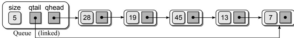
Figure 8.7: An instance of the Queue ADT implemented as a linked list.
