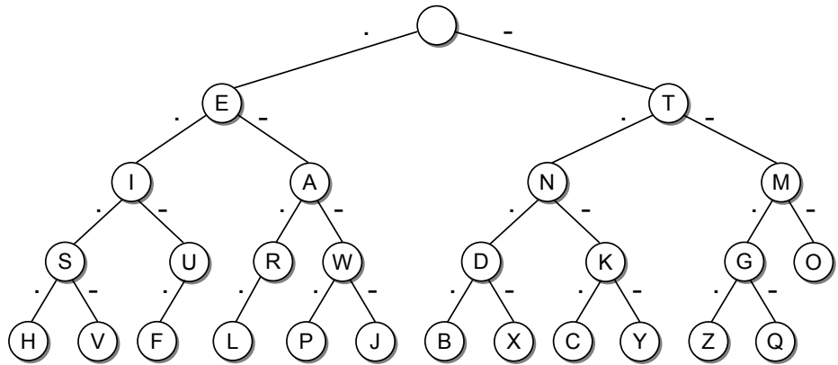
Figure 13.34: Morse Code modeled as a binary decision tree.
