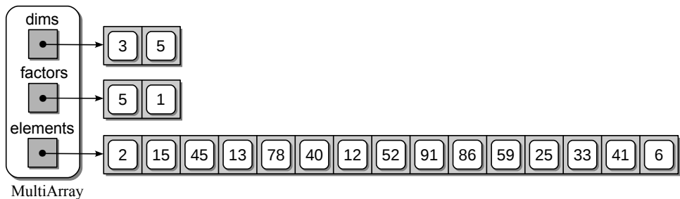
Figure 3.9: A sample MultiArray object for the 2-D array from Figure 3.6.
