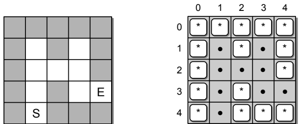
Figure 7.11: The abstract view of a maze physically represented using a 2-D array. Walls are indicated with an asterisk (*) character, while open cells contain a null reference. The start and exit cells will be identified by cell position stored in separate data fields.
