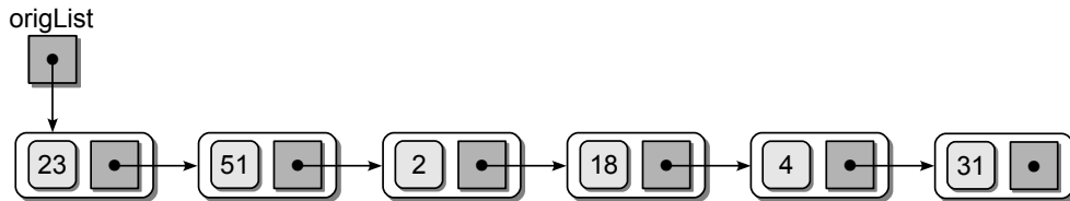
Figure 12.10: An unsorted singly linked list.
