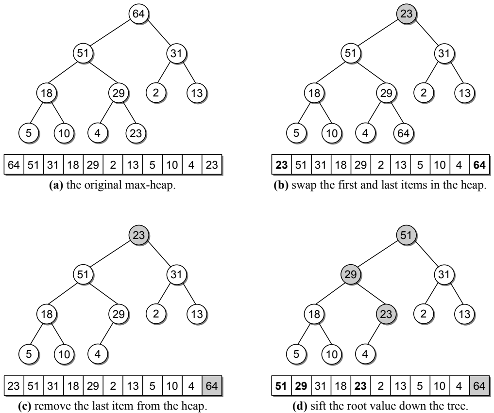
Figure 13.32: The three steps performed to extract in place a single value from the heap.
