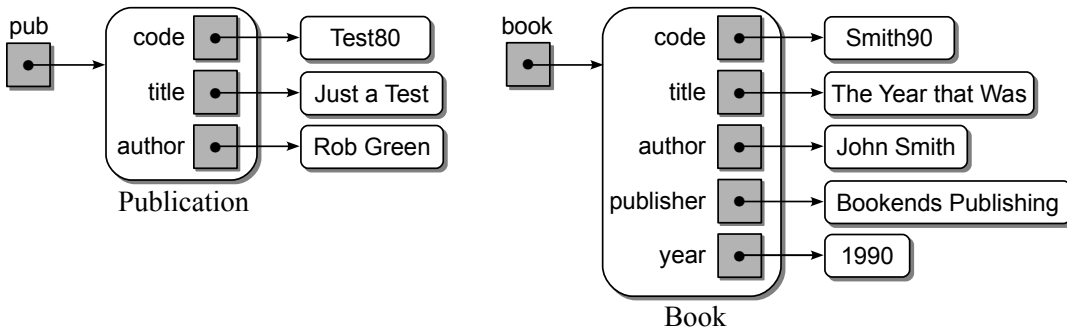
Figure D.6: The data attributes of the Publication and Book objects.
